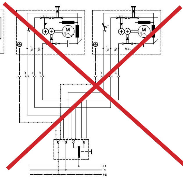
Figure 3: Inadmissible connection of two venetian blind drives using a single pole switch
